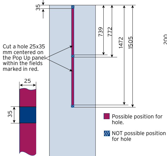
Position of holes in panel for Screen Holder/Shelf Kit
